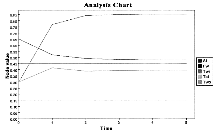
Fig. 6. Variation of values of concepts for FCM model of the five simulation steps.
