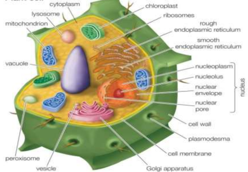
Plant cell
