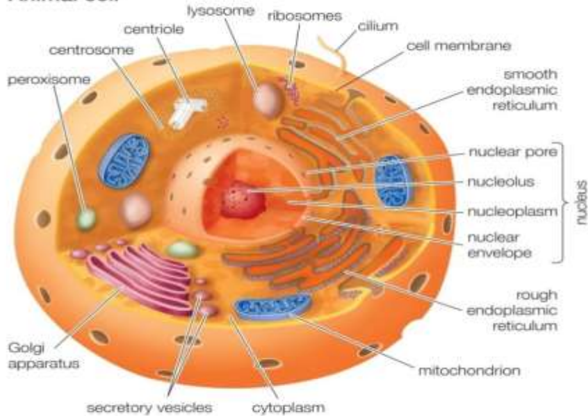
Animal cell
