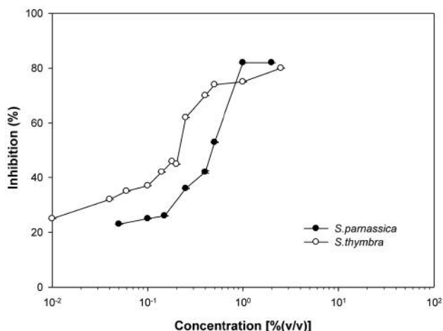
Figure 1. Antioxidant capacity of the essential oils of Satureja thymbra and S. parnassica using the 2,2-diphenyl-1-picrylhydrazyl (DPPH) free radical-scavenging method. Increasing concentrations of the essential oils of S. thymbra [0.01-2.5% (v/v)] and S. parnassica [0.05-2% (v/v)] were incubated in the presence of DPPH for 30 min. The results are shown as mean±S.D. of three independent experiments. 50% Inhibitory concentration (IC 50 ) for S. parnassica =0.4±0.3% v/v, and IC 50 for S. thymbra =0.22±0.25 % v/v.
