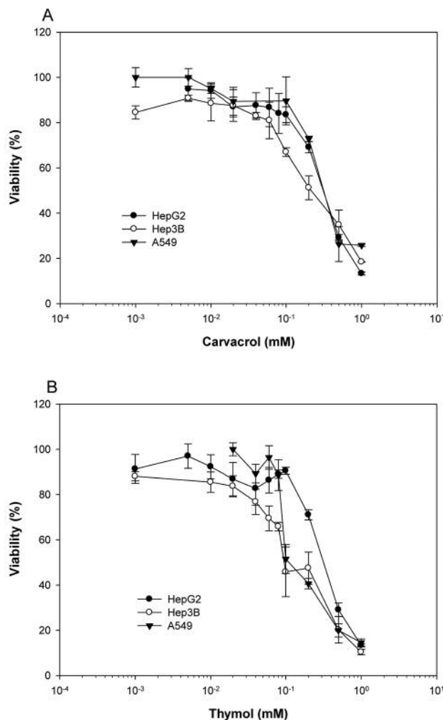
Figure 4. Antiproliferative activity of carvacrol (A) and thymol (B). Cells were incubated with increasing concentrations of carvacrol, and thymol (0.001-1 mM) for 72 h. Estimation of cell viability was determined by the sulforhodamine B assay. The results are shown as the mean±S.D. of three independent experiments.
