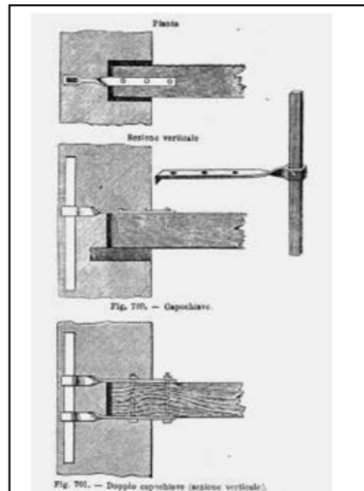
Figure 3 : Connection between beam and masonry with single and double steel element and punch, Pareto and Sacheri (1889).
