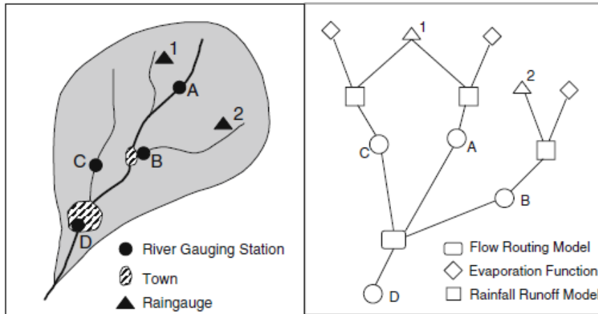
Example of model configuration in a flood forecasting system (Sene 2008)
