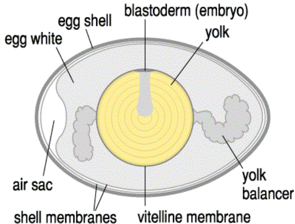
Structure of the fertilized hen's egg when laid
