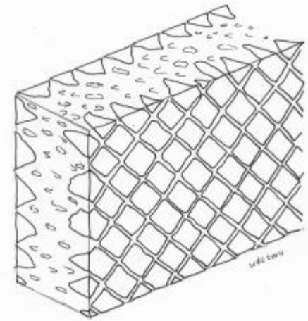
Opus quasi reticulatum
