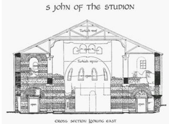
CROSS SECTION looking east
