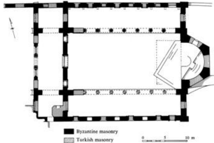
Figure 5. Studios Basilica. Plan
