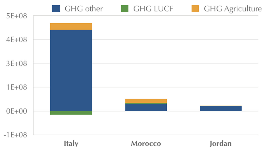
Fig. 3. Baseline for the indicator GHG emissions (Italy, Morocco and Jordan are reported as an example). LUCF = Land Use Change and Forestry .
